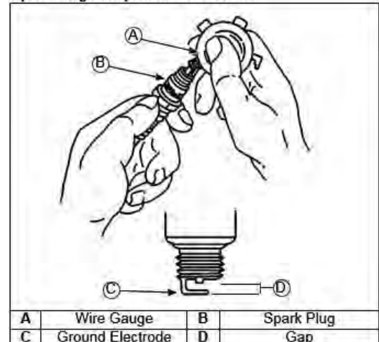
Spark Plug Component and Details
